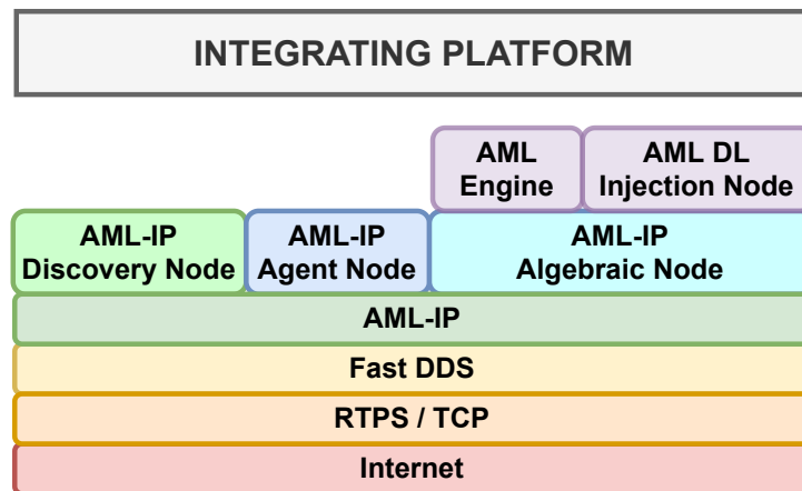
Figure 3: AML-IP layer model.
